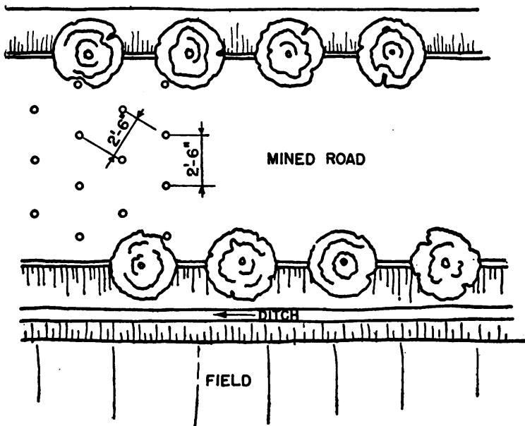
FIGURE 60.—Tellermine road and track blocks.
